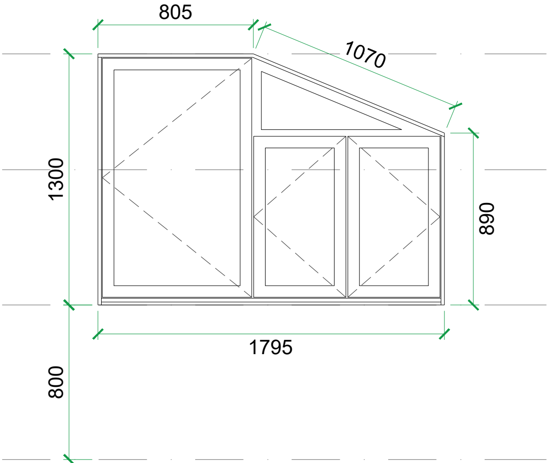
W02 Bedroom 2 Aluminium framed with 3x side opening casements, and one fixed triangular pane.
