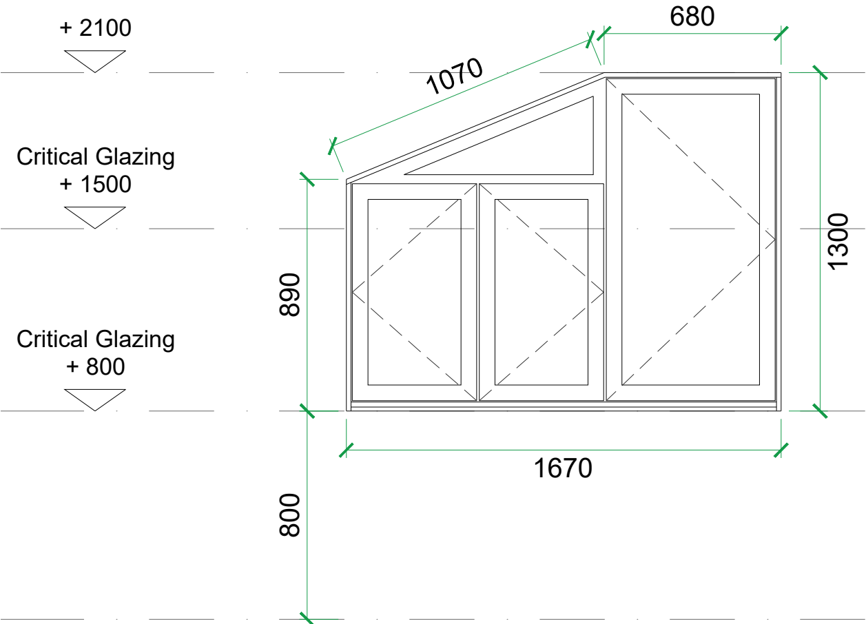
W01 Bedroom 3 Aluminium framed with 3x side opening casements, and one fixed triangular pane.
