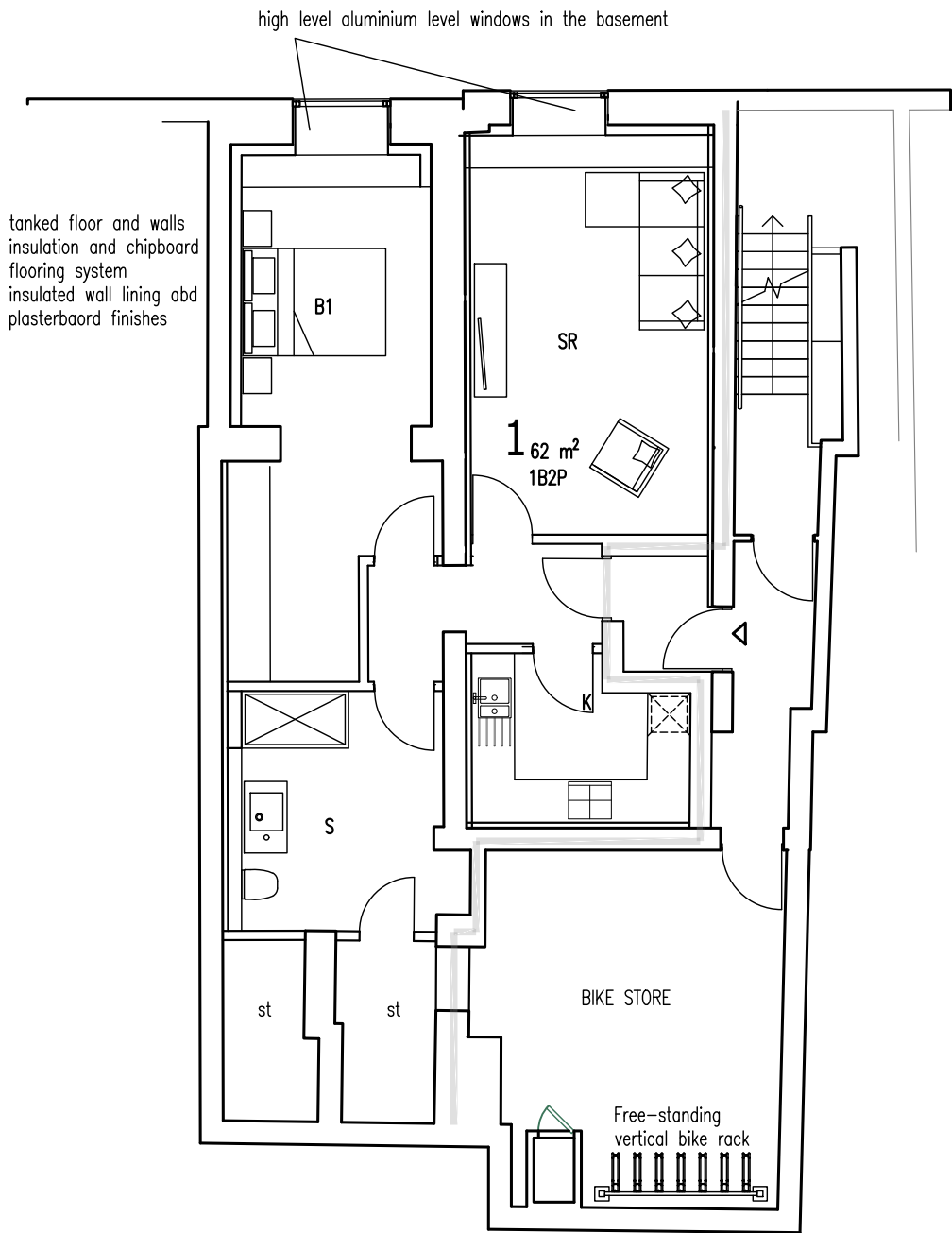
Basement Floor Plan @ 1/100
