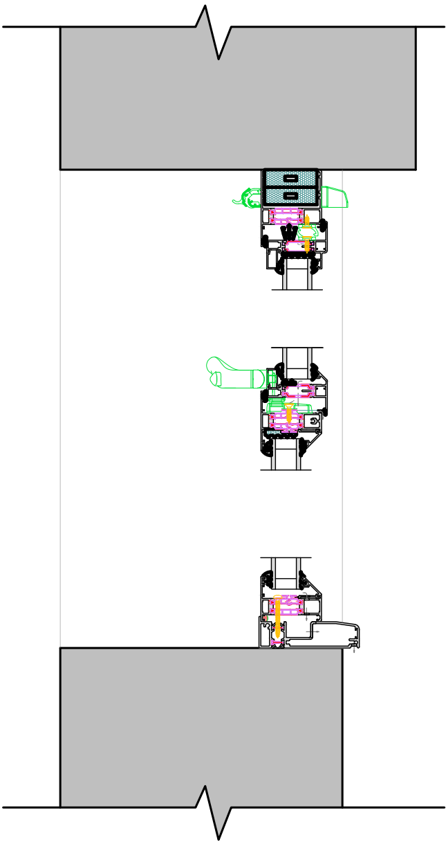
Window Section Detail @ 1/5
