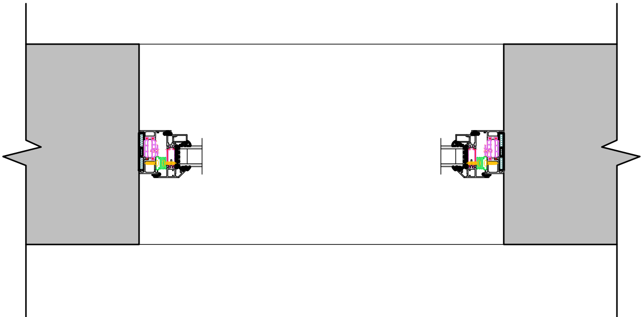
Window Jamb Detail @ 1/5
