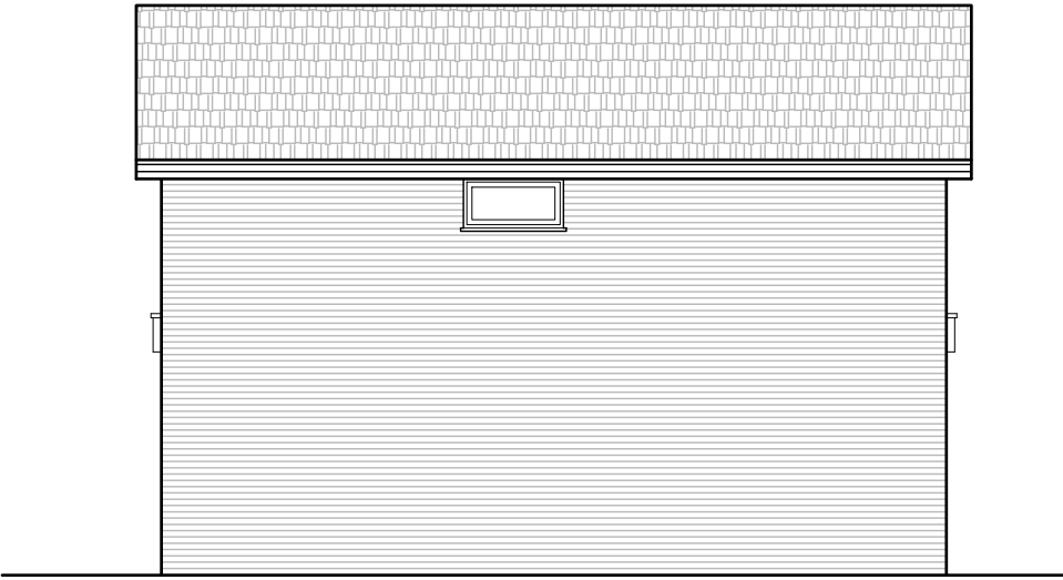
PROPOSED REAR ELEVATION - NO CHANGE 1:100
