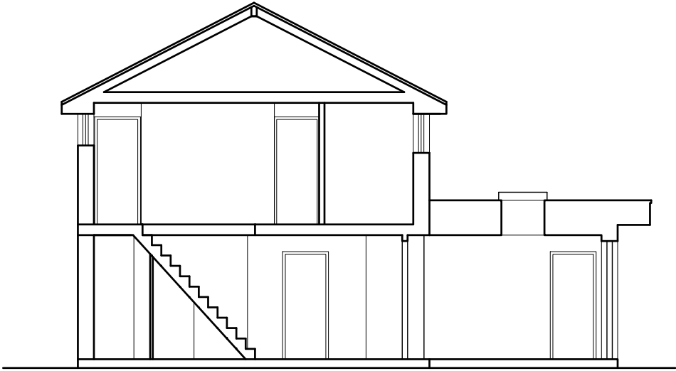
PROPOSED SECTION A-A 1:100
