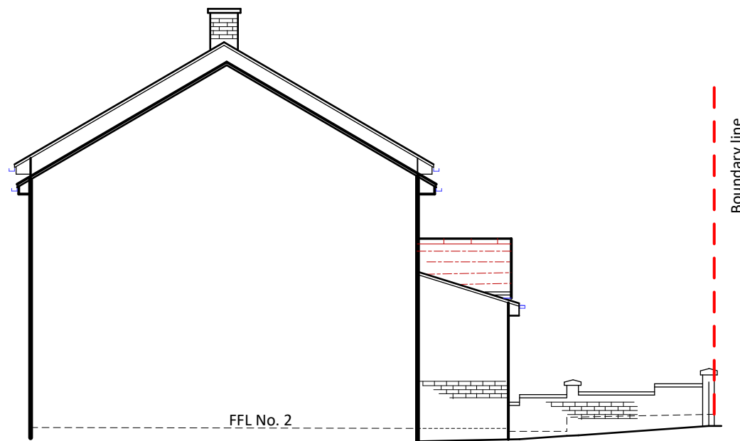
SIDE
