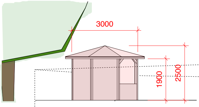
Side Elevation - Gazebo
