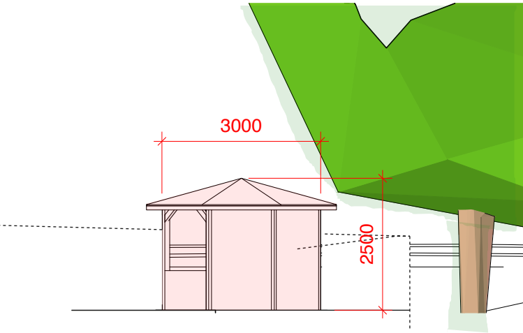
Side Elevation - Gazebo
