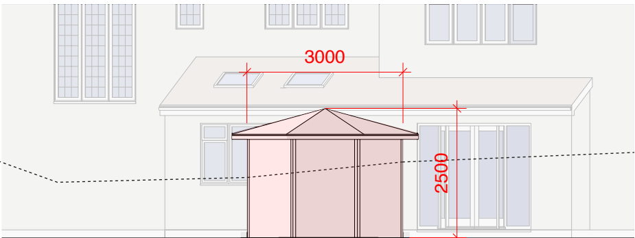
Rear Elevation - Gezebo
