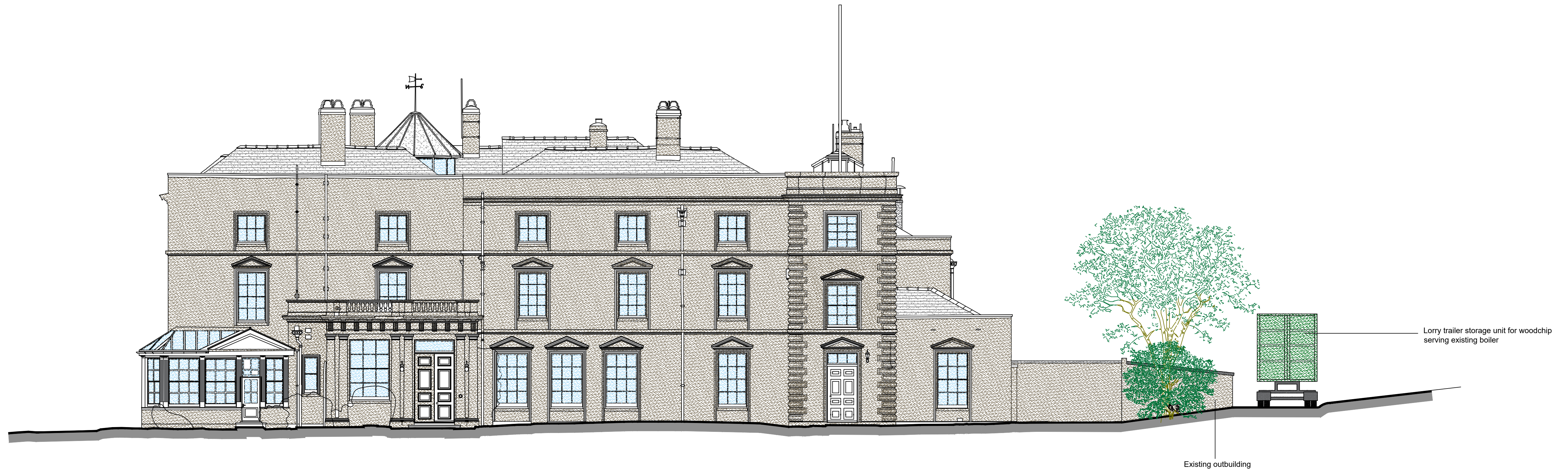
Existing West Elevation 1:100
