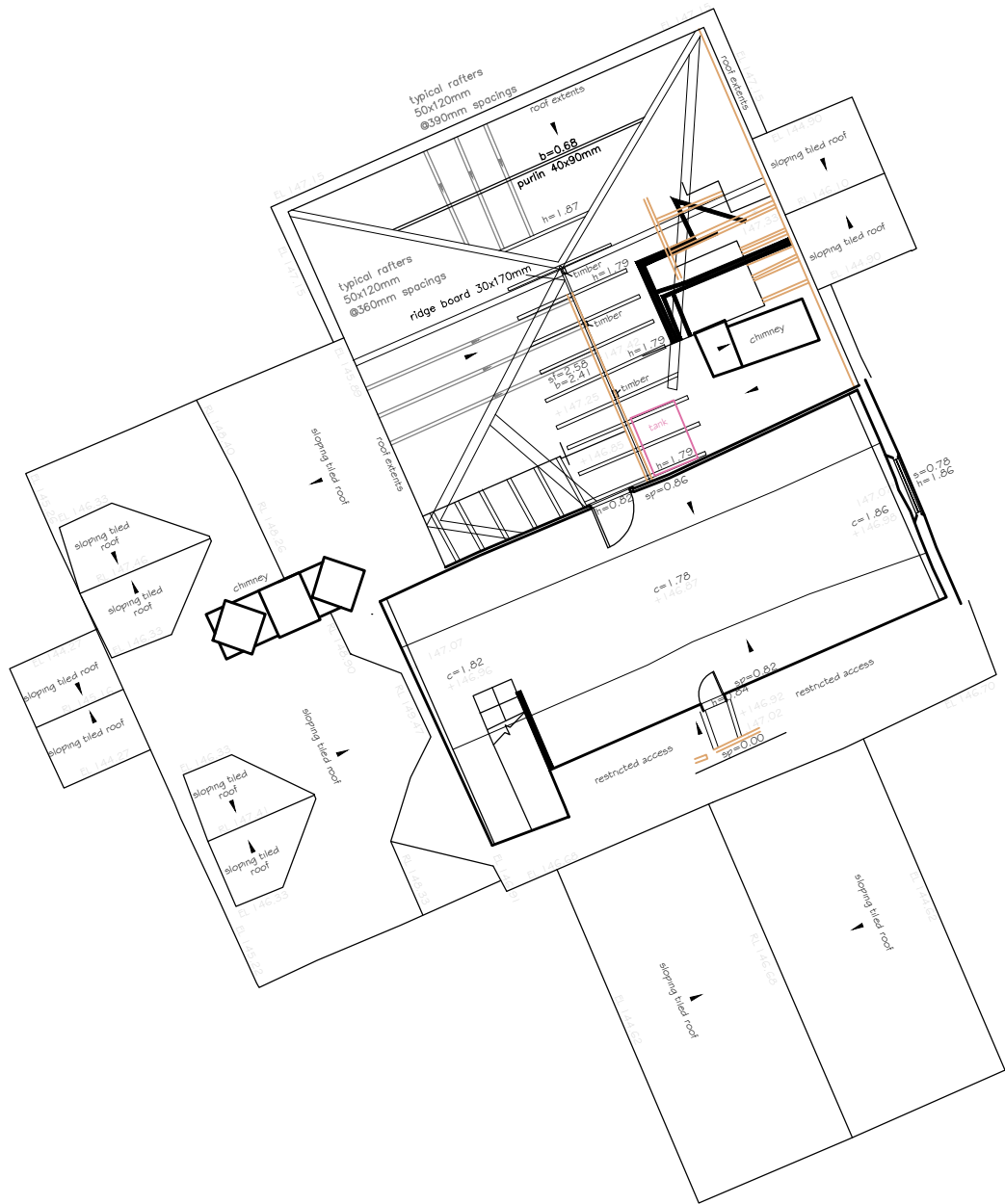
Loft Plan @ 1/100
