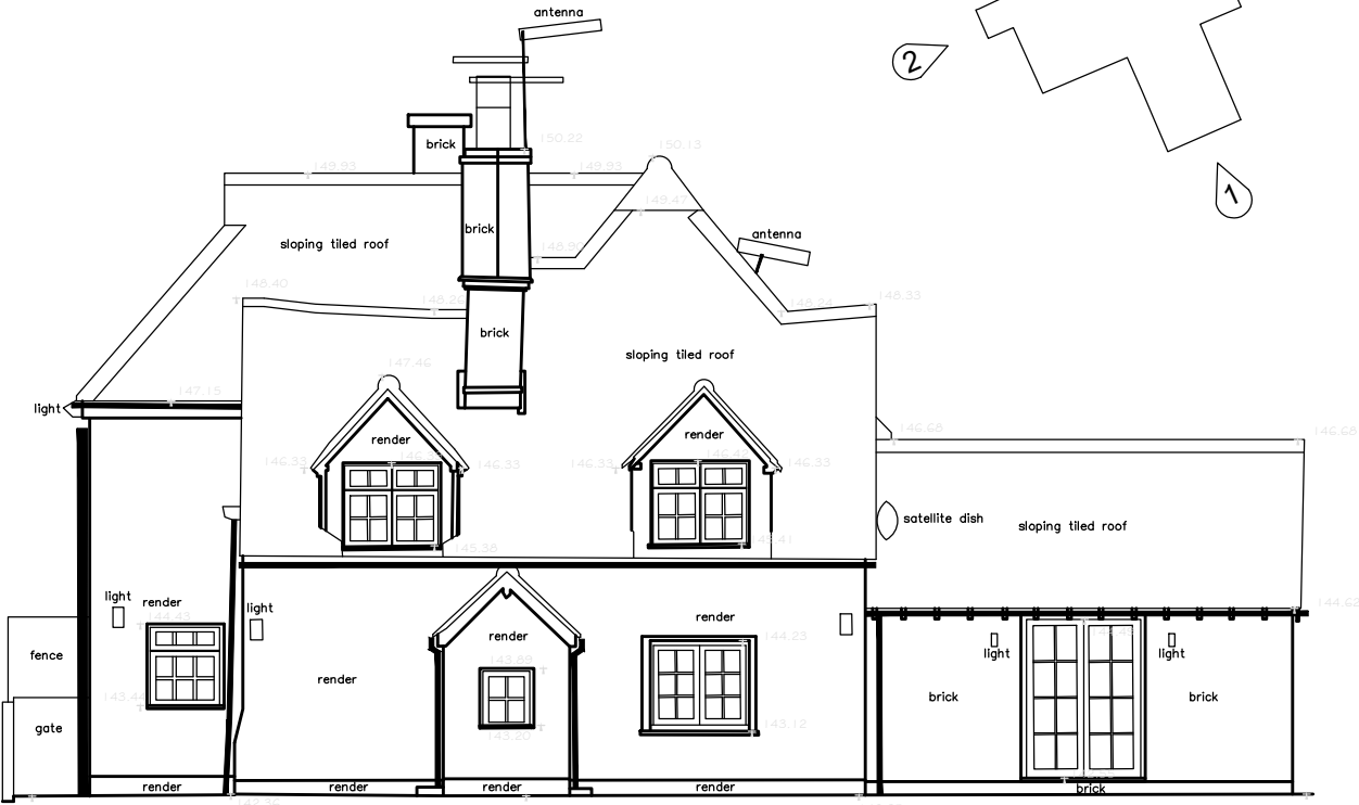
Elevation 2 @ 1/100
