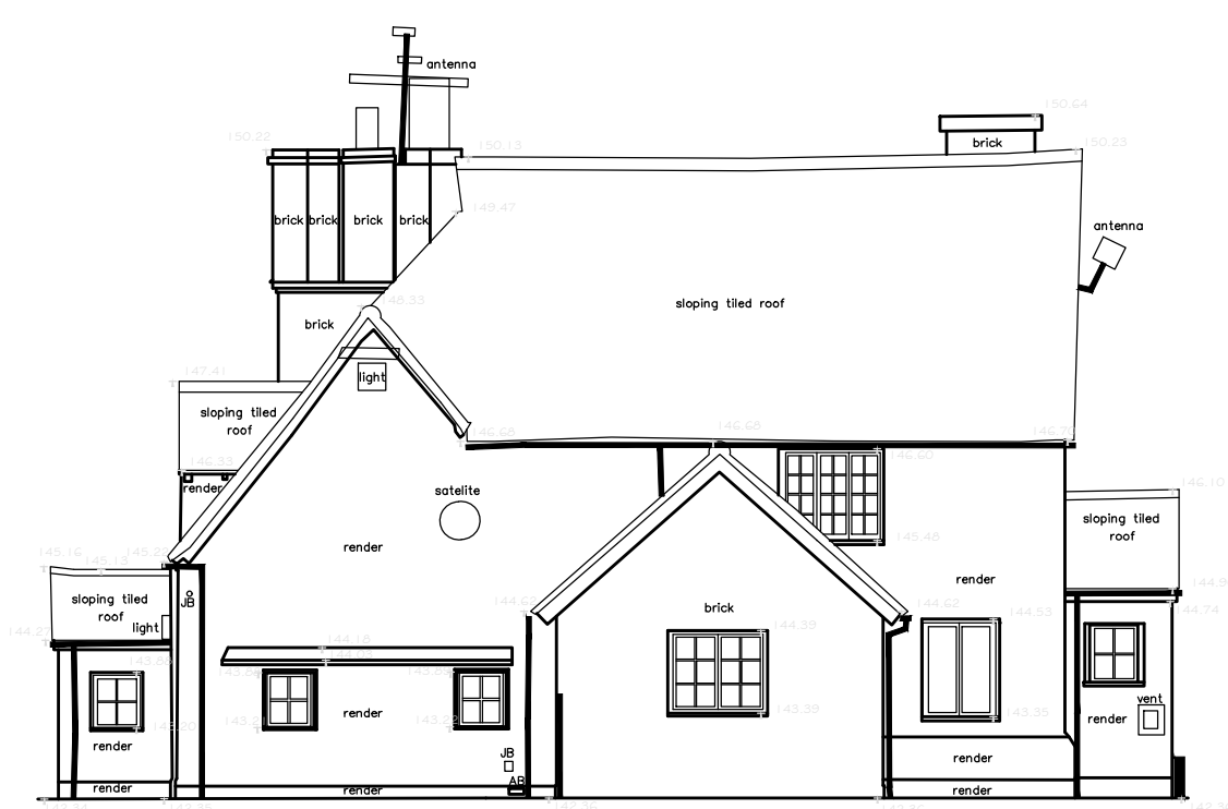
Elevation 1 @ 1/100
