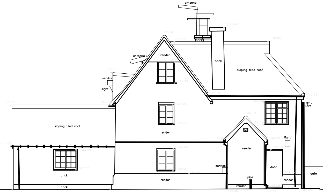
Elevation 4 @ 1/100
