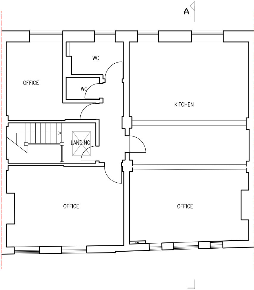
SECOND FLOOR PLAN SCALE 1/100
