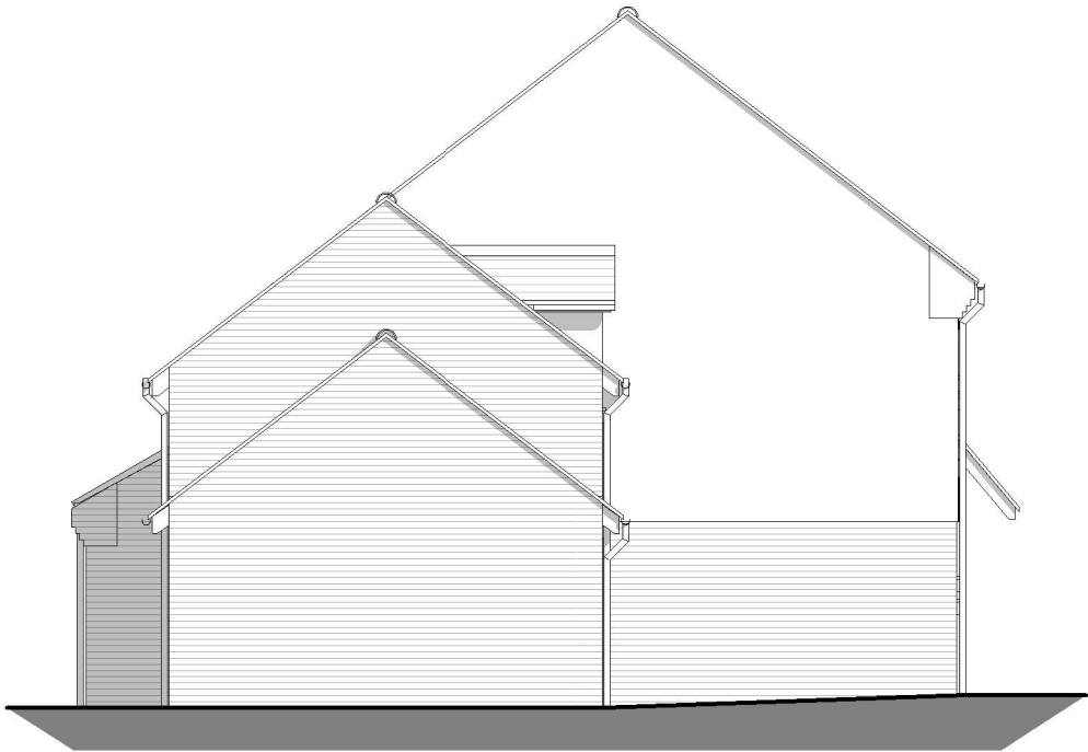
Existing Side A Elevation 1 : 100
