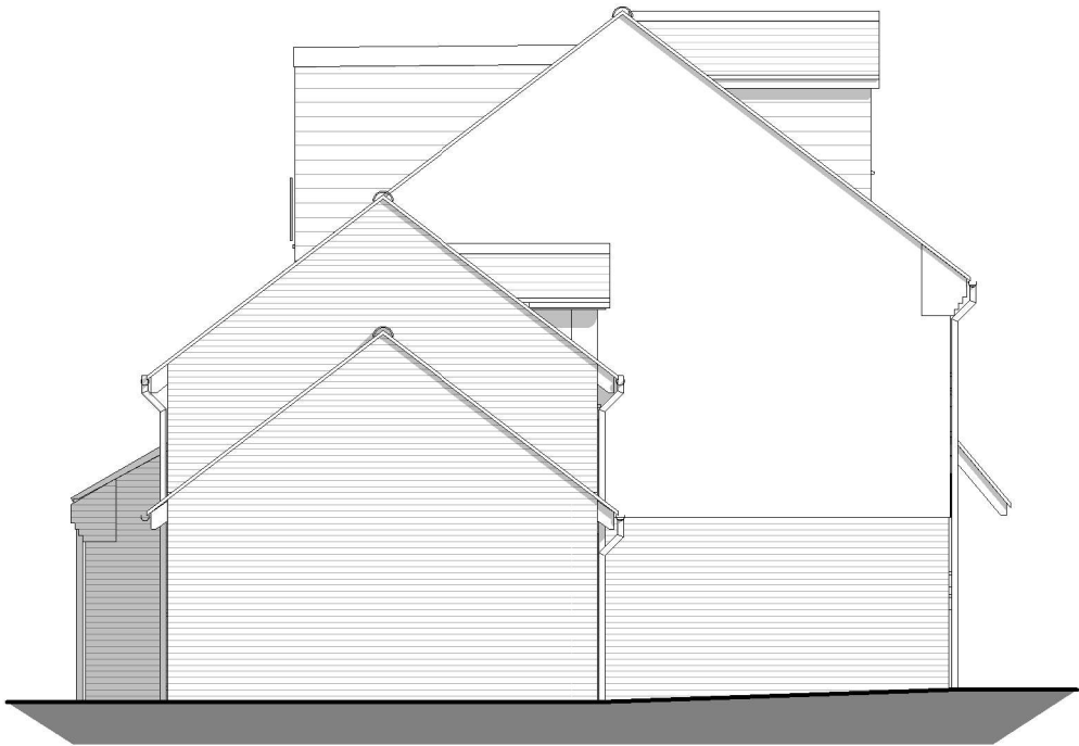
Proposed Side A Elevation 1 : 100
