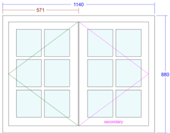
1. Conventional Cottage Window (Window 1)
