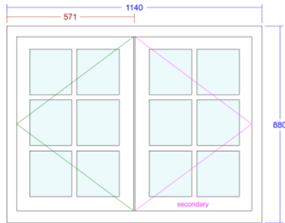
2. Conventional Cottage Window (Window 2)
