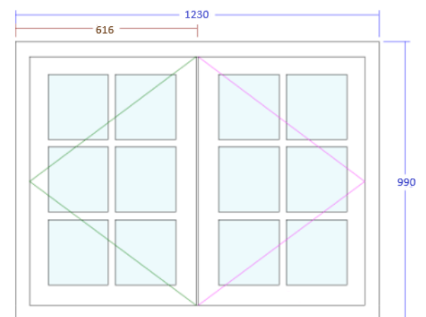
6. Sealed close Cottage Window (Window 6) 26x23, 99x123
