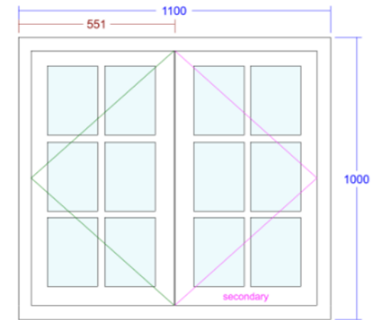
3. Conventional Cottage Window (Window 3)
