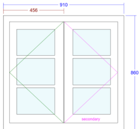
4. Conventional Cottage Window (Window 4)
