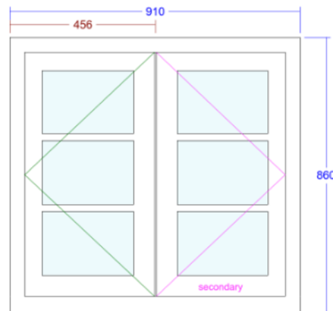
5. Conventional Cottage Window (Window 5)
