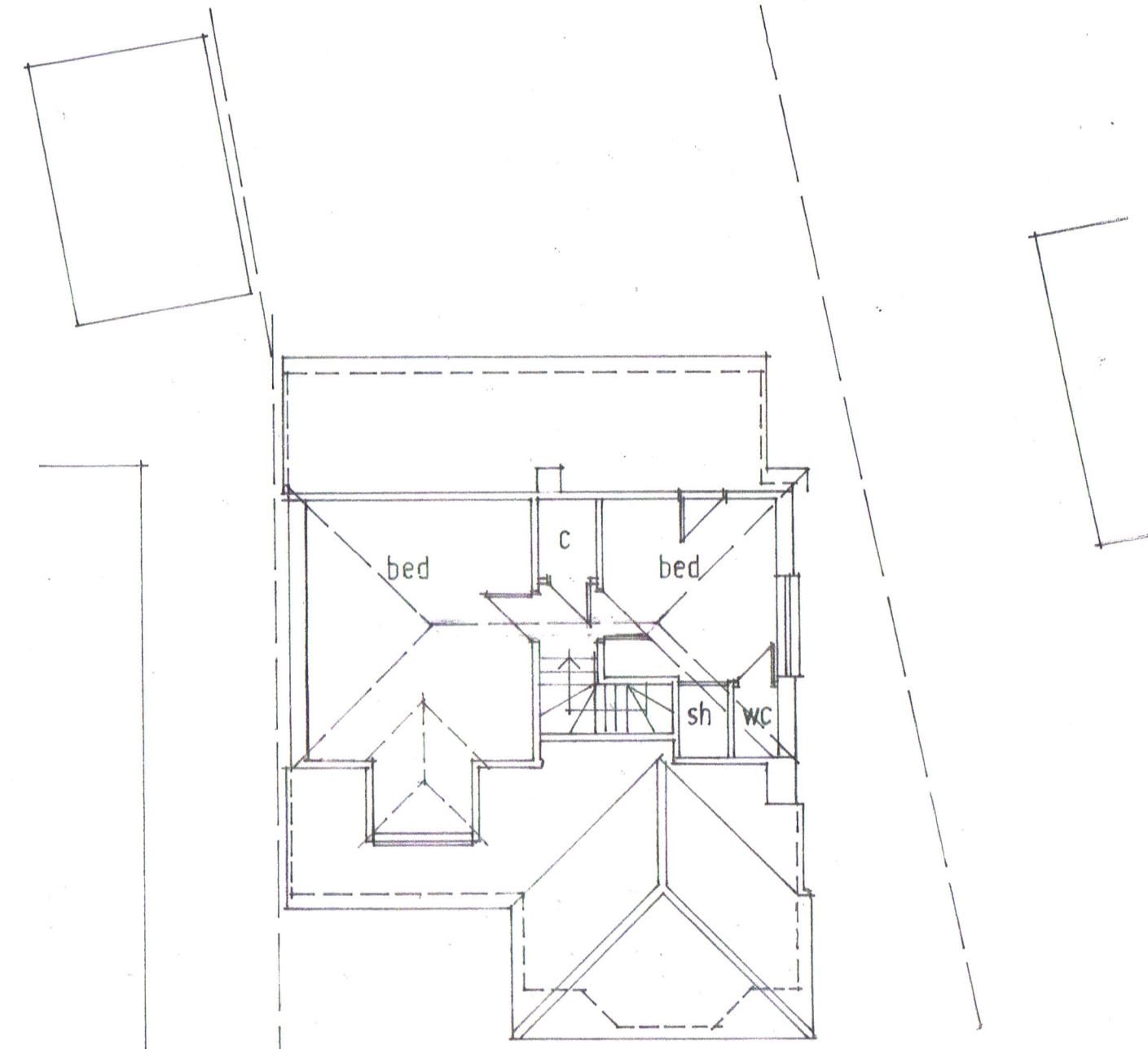
FIRST FLOOR
