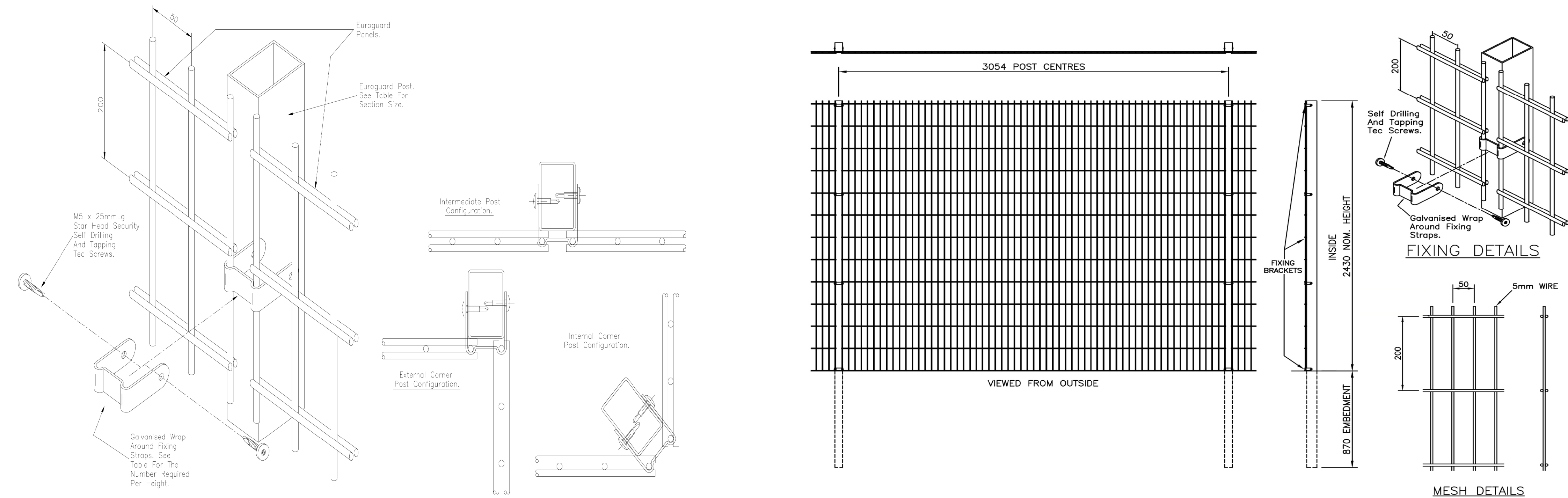
Typical Fixing Details:
