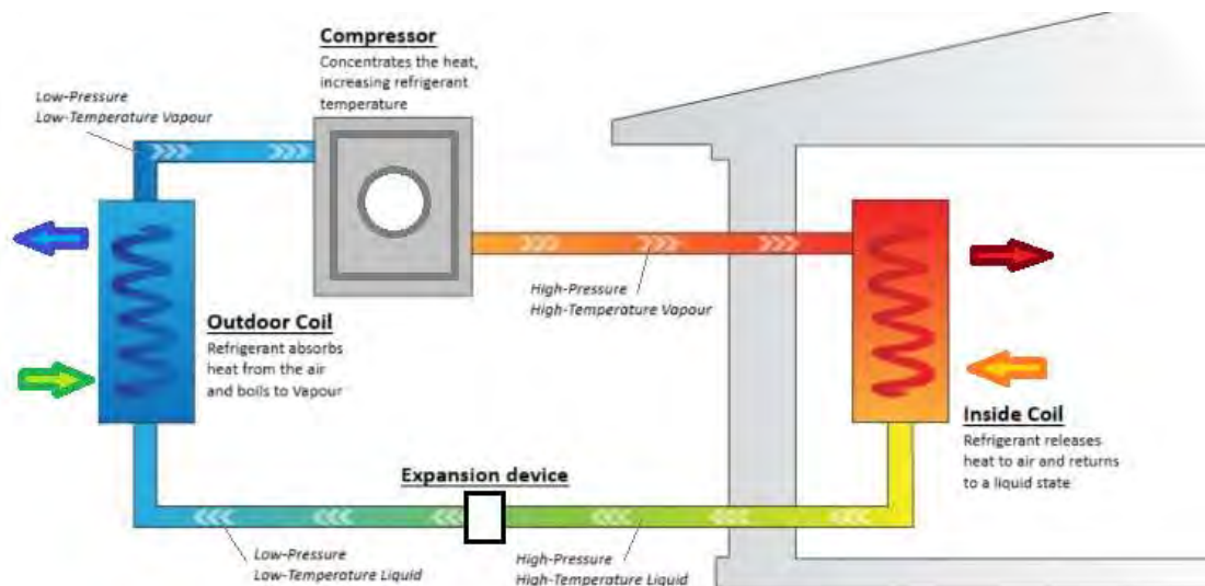
Figure 8 – Air Source Heat Pump – Typical Diagram
