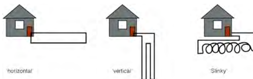
Figure 15 – Ground Source Heat Pump Loop Arrangements
