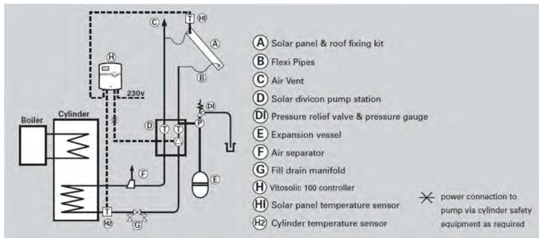
Figure 14 – Evacuated Tube Solar Collector Typical Schematic Diagram
