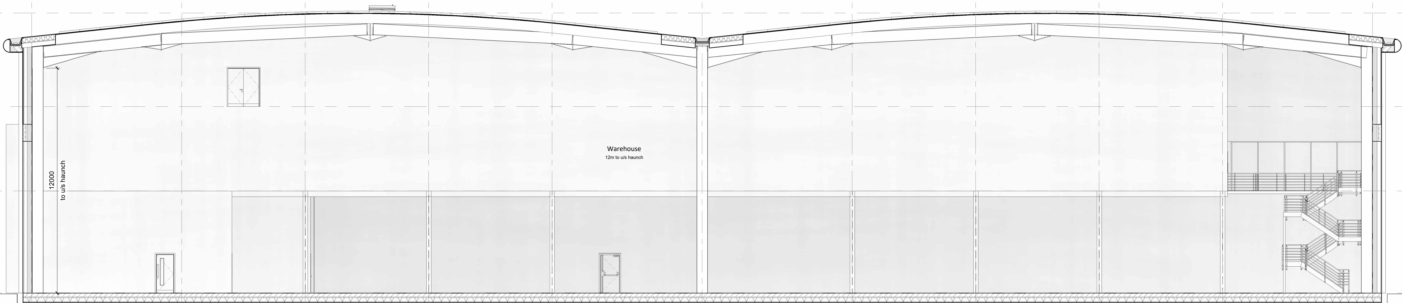
Unit 3 - GA Section B-B
