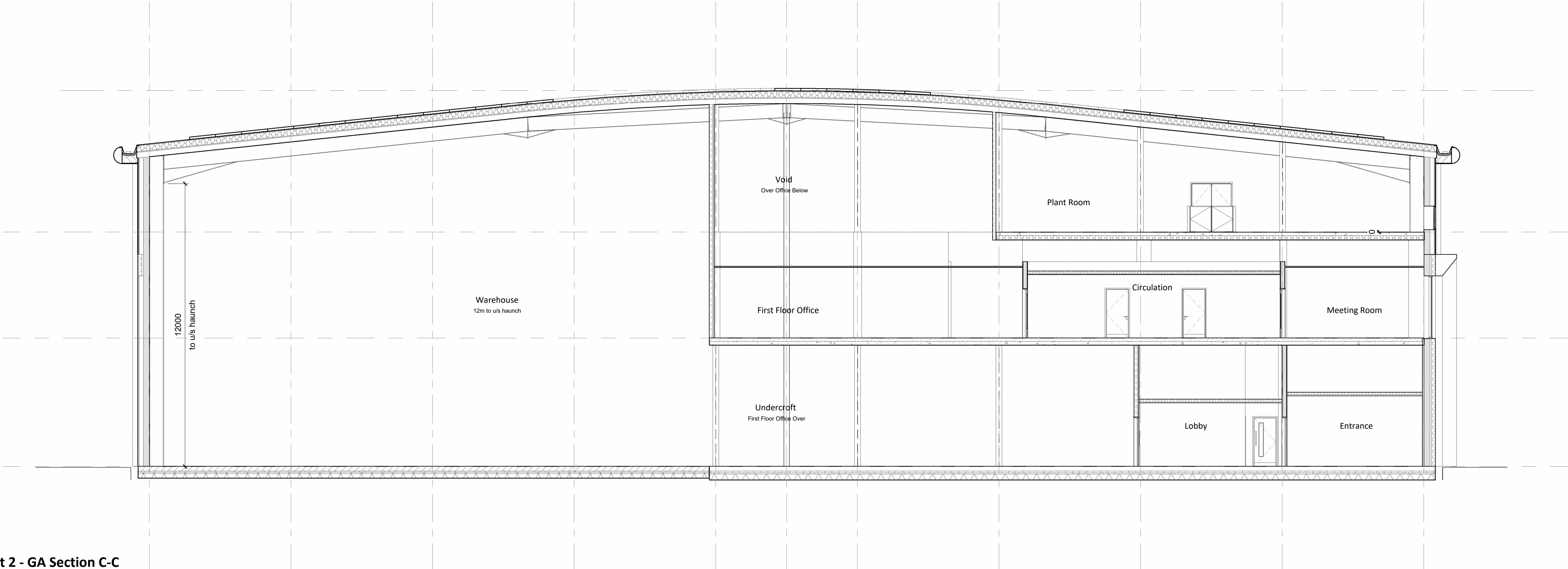
Unit 2 - GA Section C-C
