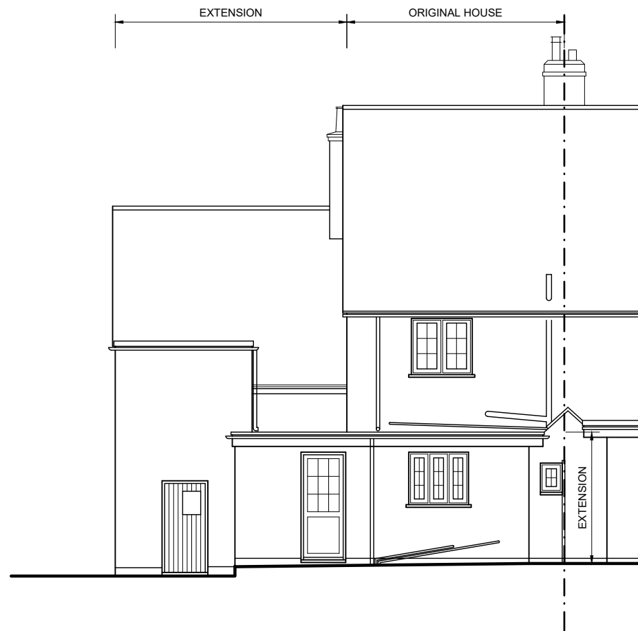
Rear Elevation
