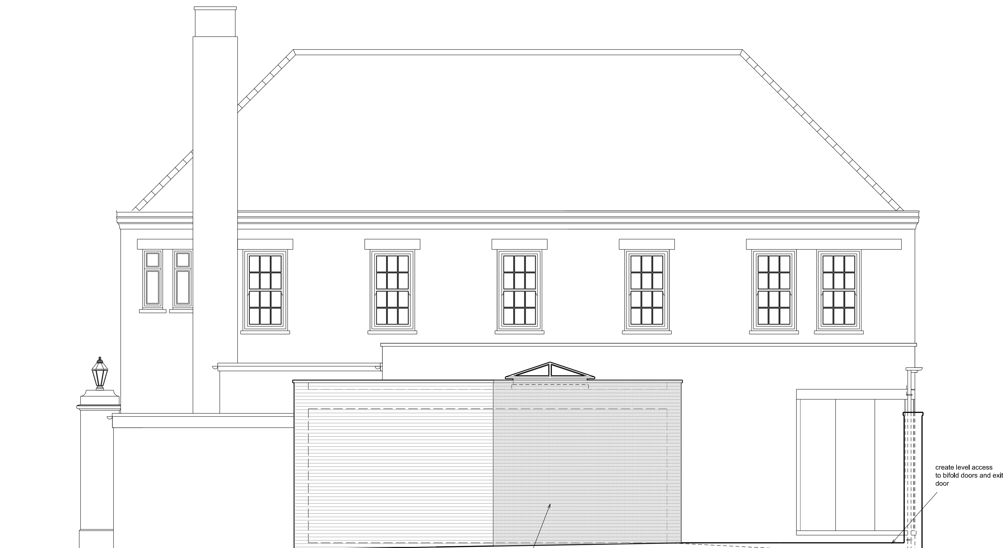
new single storey extension, comprising of new cavity wall construction with facing brick to match existing, with parapet walls to the perimeter, flat roof in a grp finish, with feature roof lantern, with bifold doors to access patio
