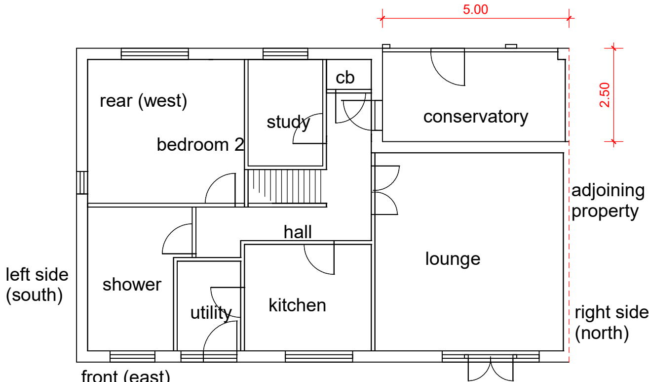
front (east) GROUND FLOOR LAYOUT
