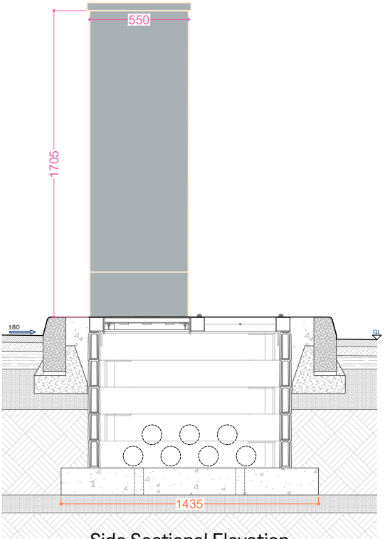
Side Sectional Elevation
