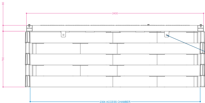
Rear Sectional Elevation
