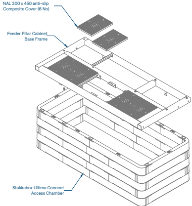
NAL Cabinet Base System – Schneider LV Pillar Cabinet Base
