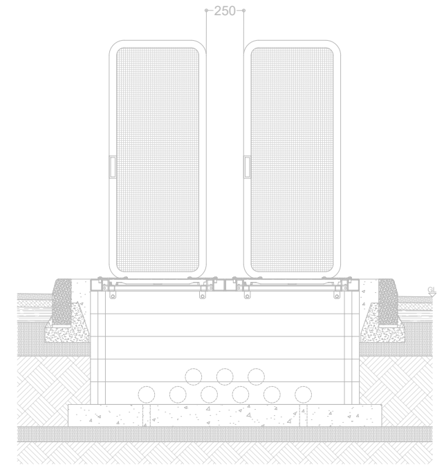
Side Sectional Elevation
