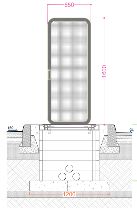
Side Sectional Elevation
