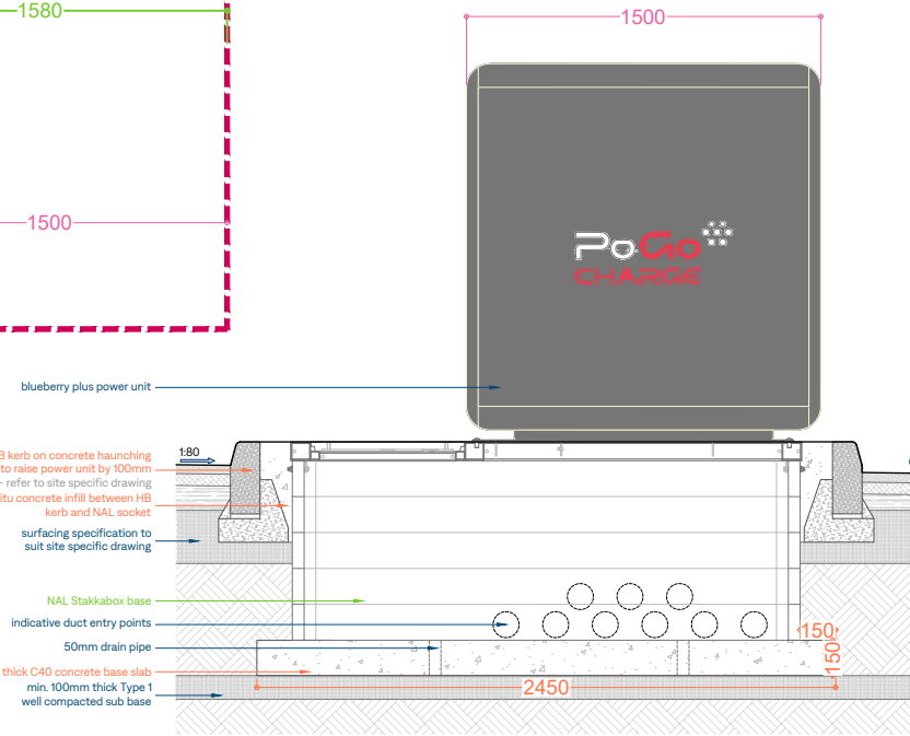
Front Sectional Elevation
