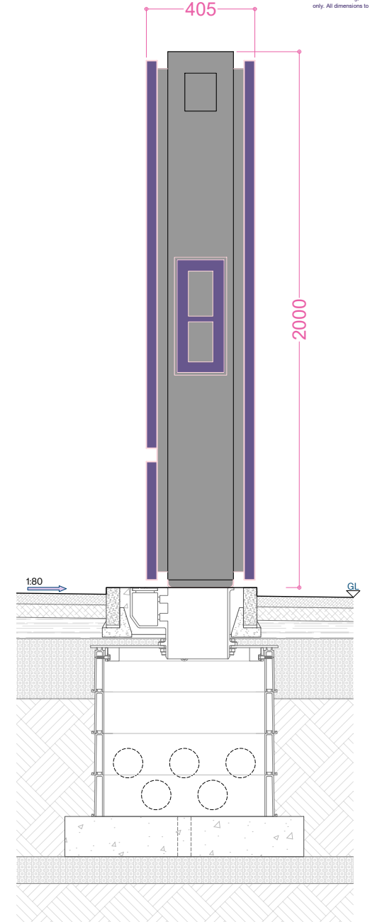
Side Sectional Elevation
