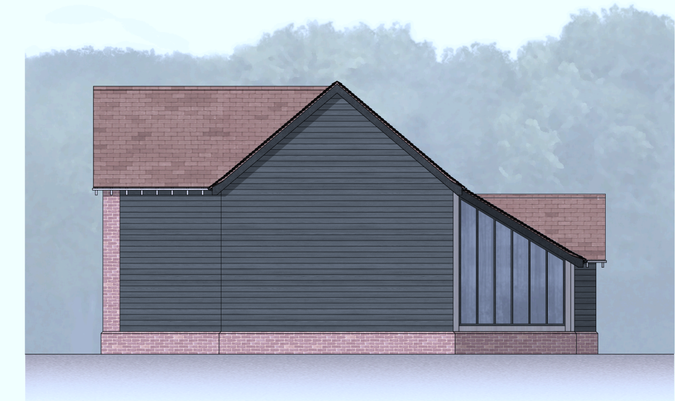
Side Elevation
