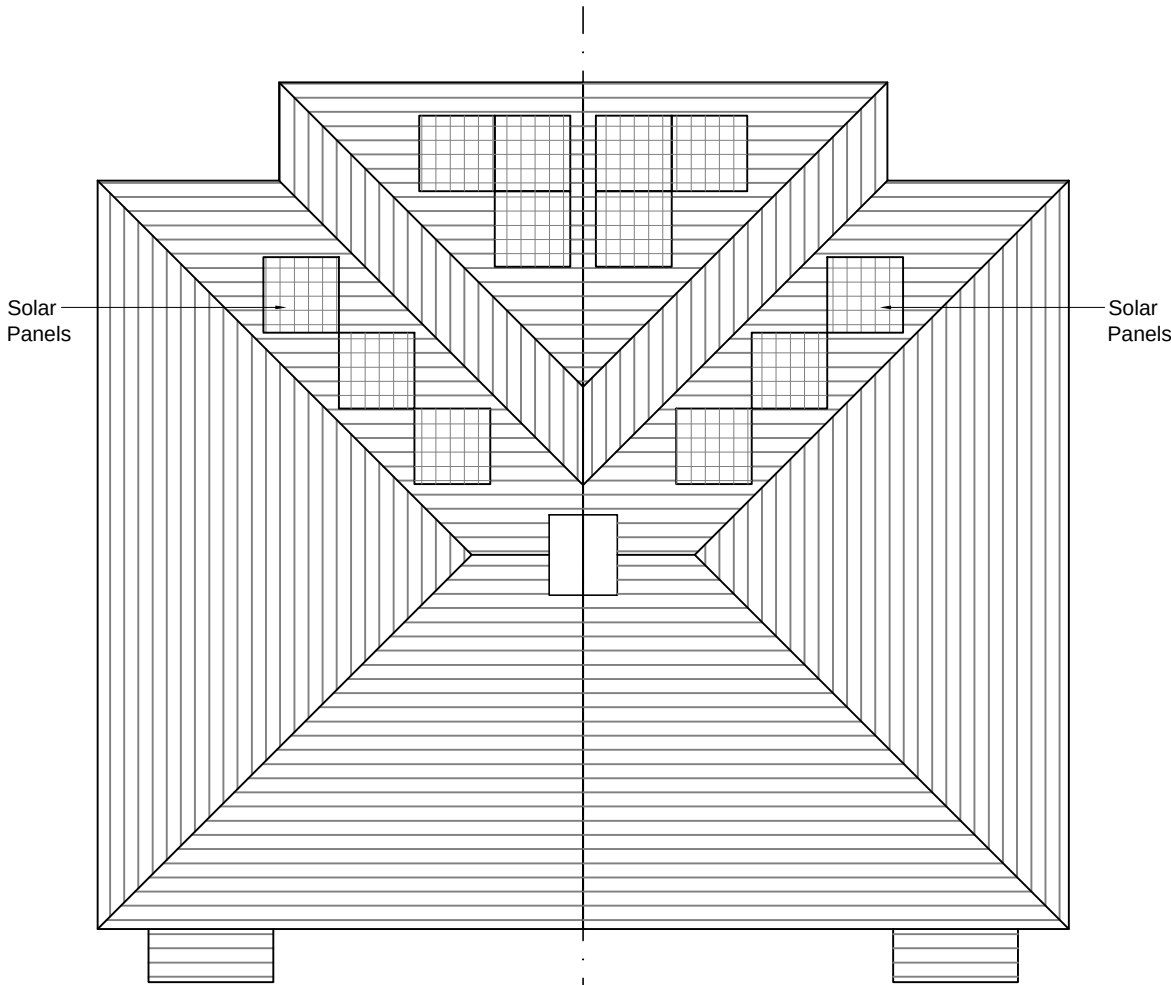
Roof Plan
