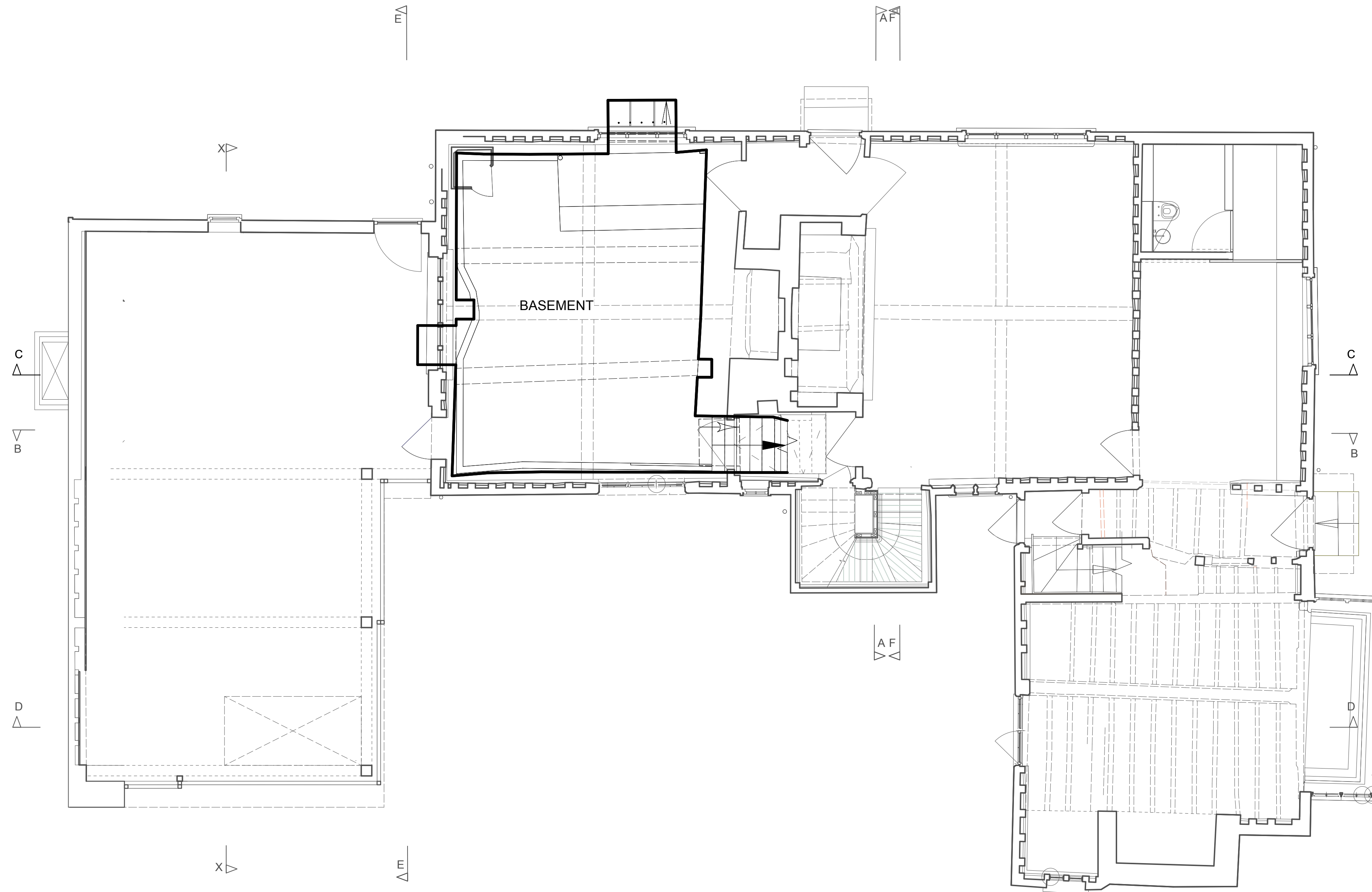
GROUND FLOOR PLAN AS PROPOSED SHOWN IN GREY FOR REFERENCE
