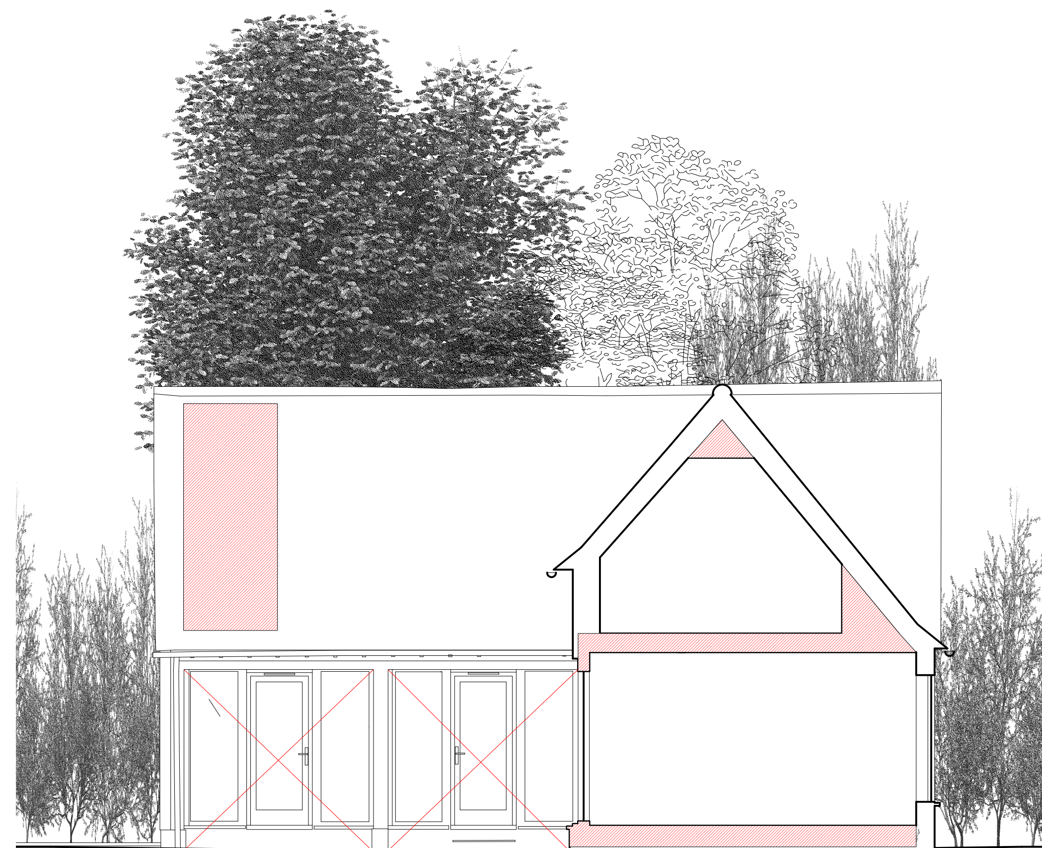
SECTION ee AS EXISTING
