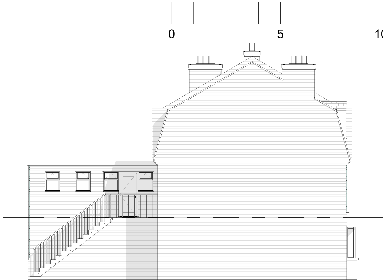
3 West Elevation 1 : 100
