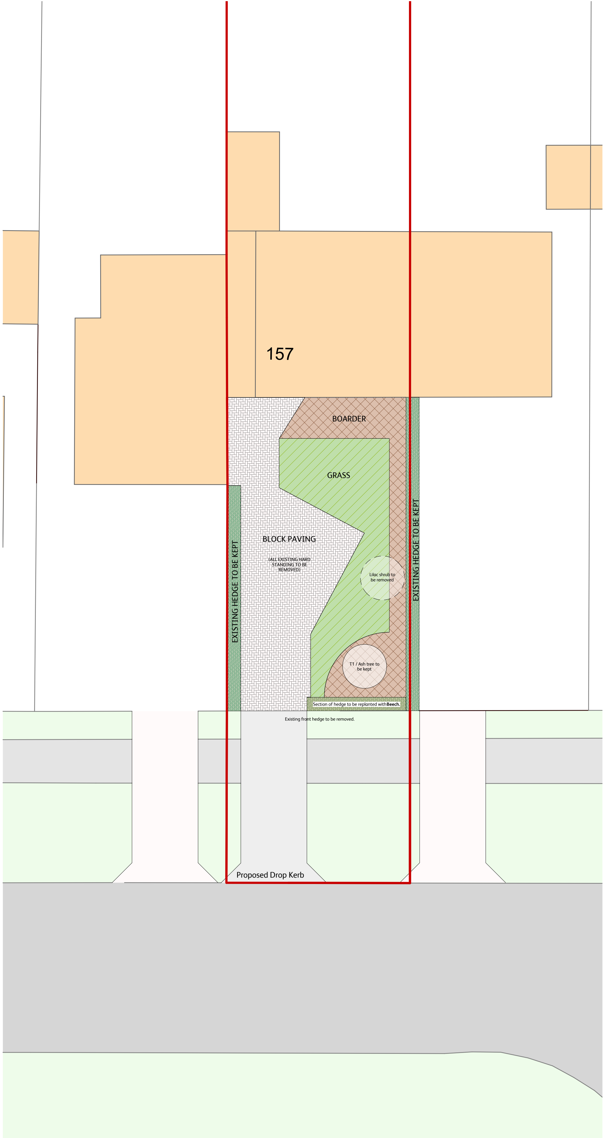
2 Proposed 1 : 100
