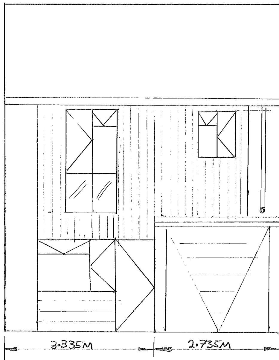
FRONT ELEVATION
