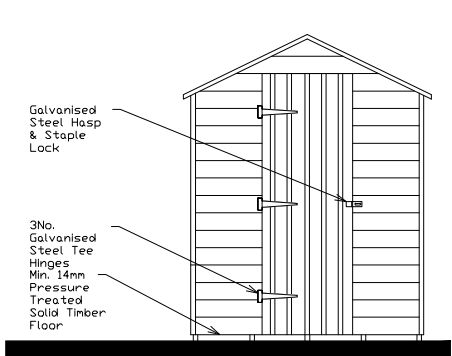
Front Elevation 1 : 50
