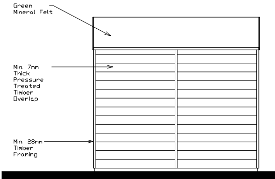
Side Elevation - Left 1 : 50
