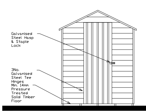
Front Elevation 1 : 50
