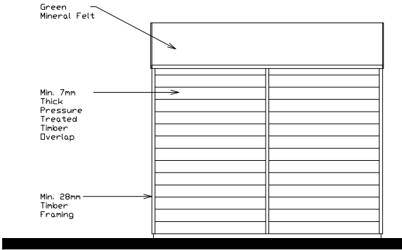
Side Elevation - Left 1 : 50
