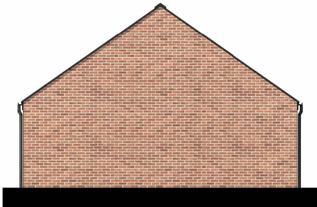
Side Elevation - Right 1 : 100
