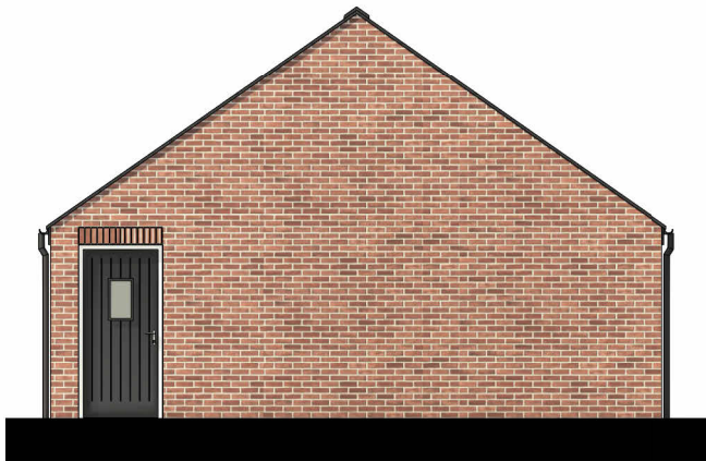
Side Elevation - Left 1 : 100
