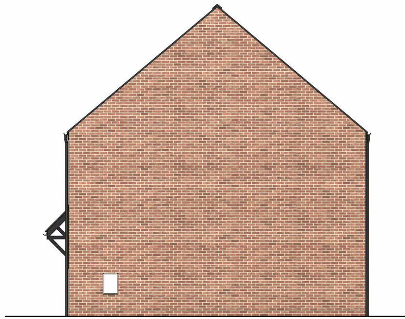
Side Elevation - Right 1 : 100
