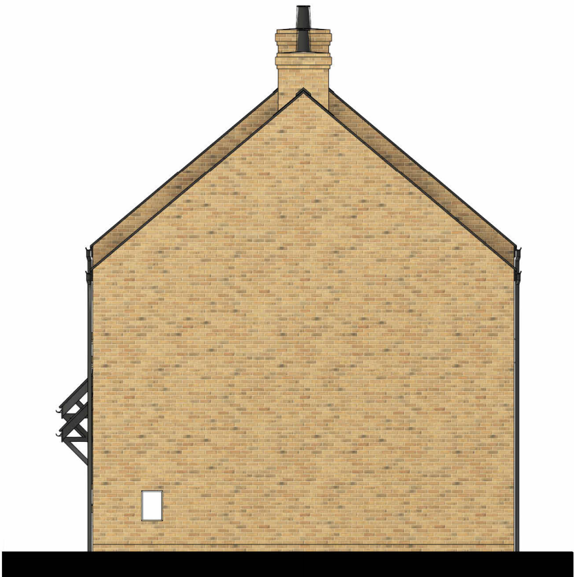
Side Elevation - Right 1 : 100
