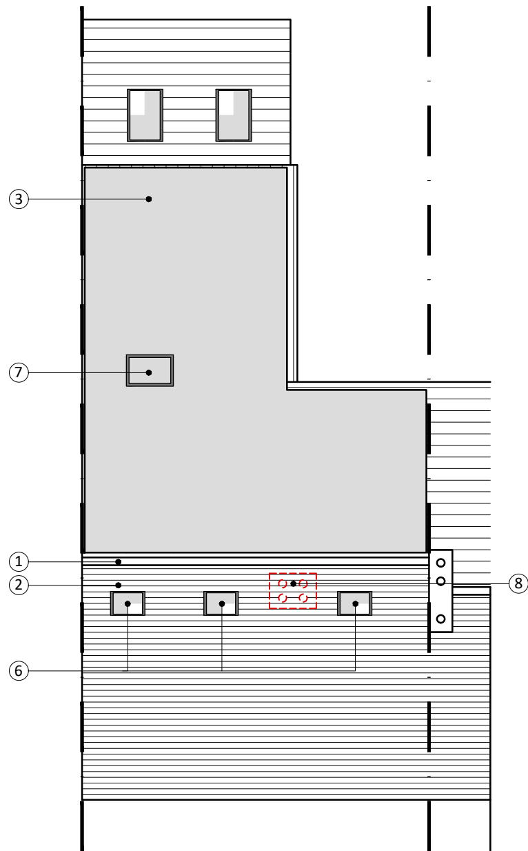
ROOF PLAN
