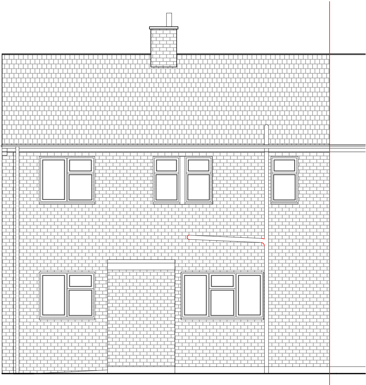
END OF TERRACE REAR ELEVATION
