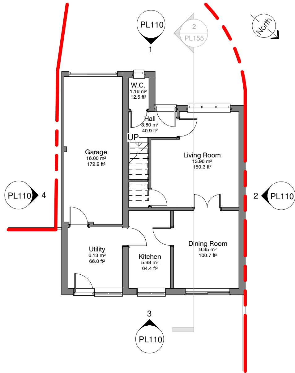
1 GROUND - Existing 1 : 100 @A3
