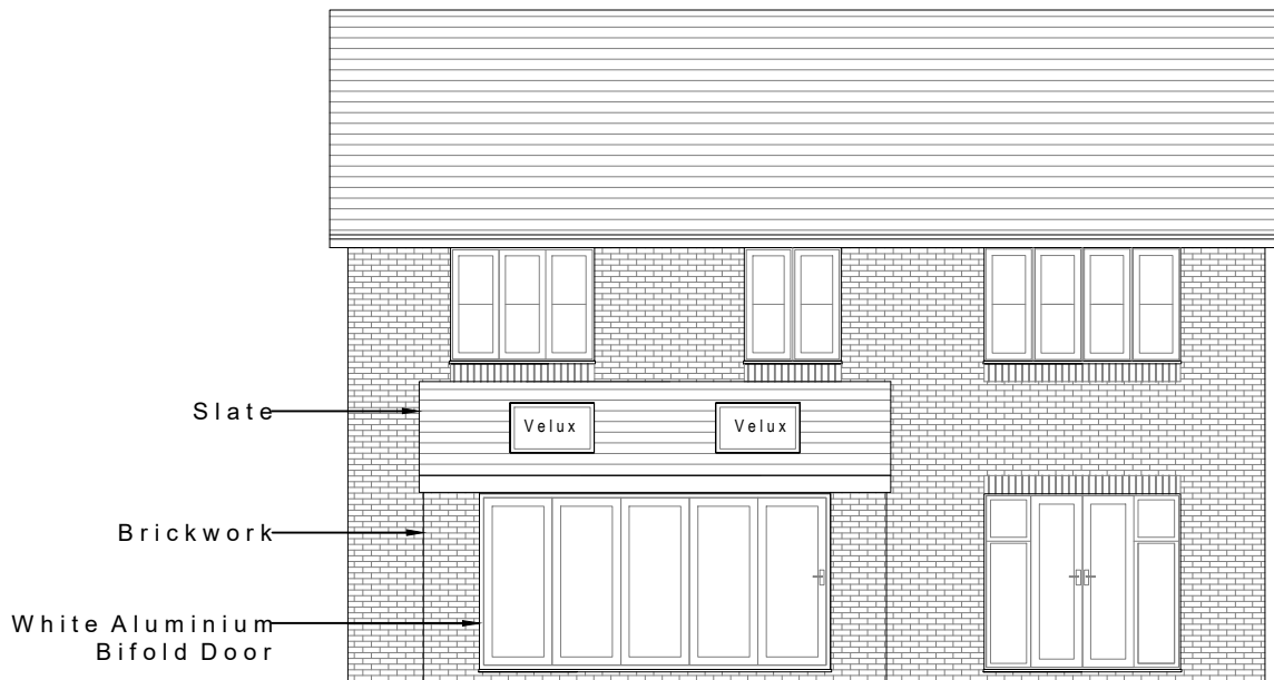
Rear Elevation
