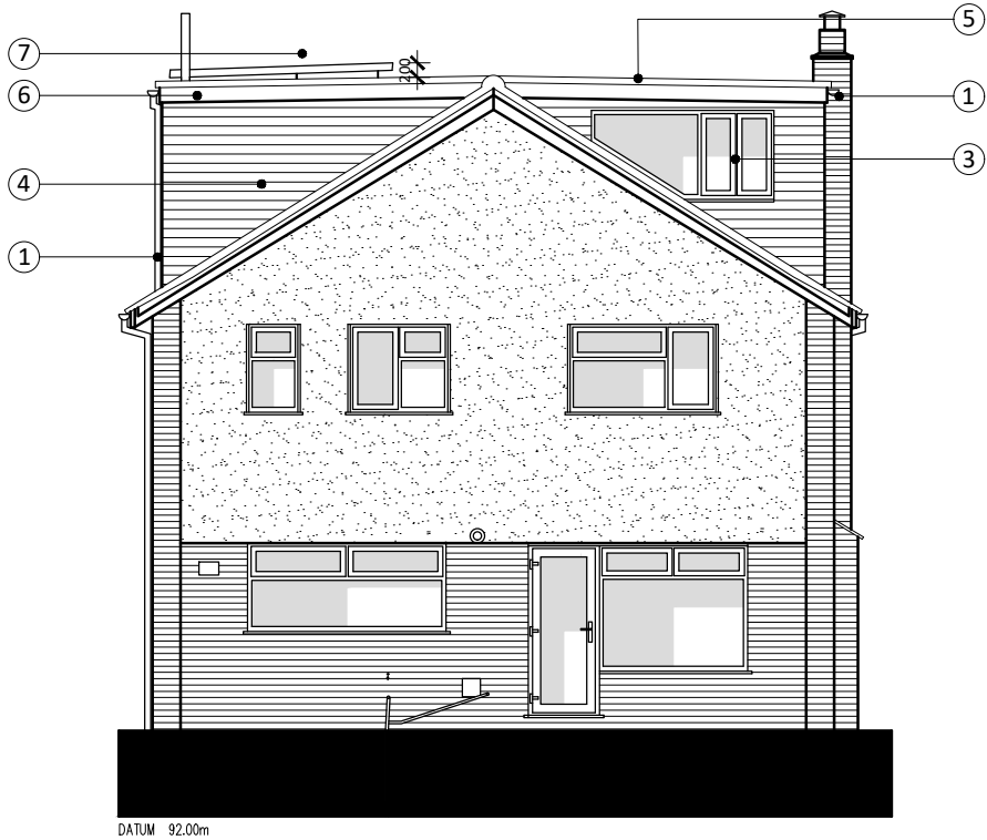
REAR ELEVATION (C-C)
