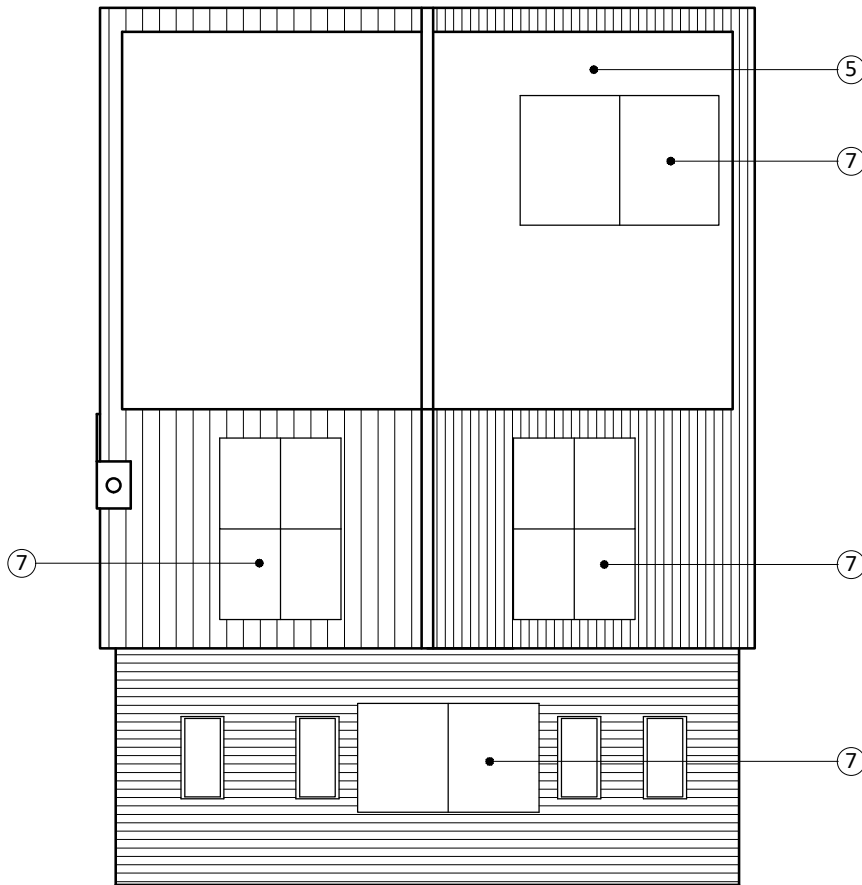
ROOF PLAN
