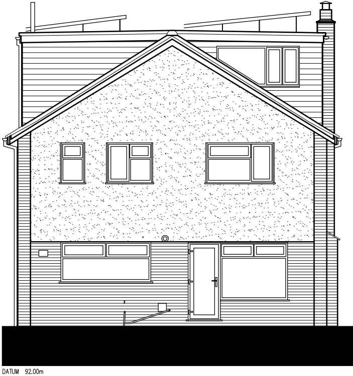
REAR ELEVATION (C-C)
