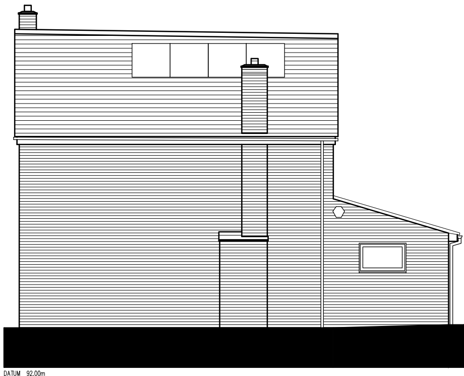
SIDE ELEVATION (B-B)
