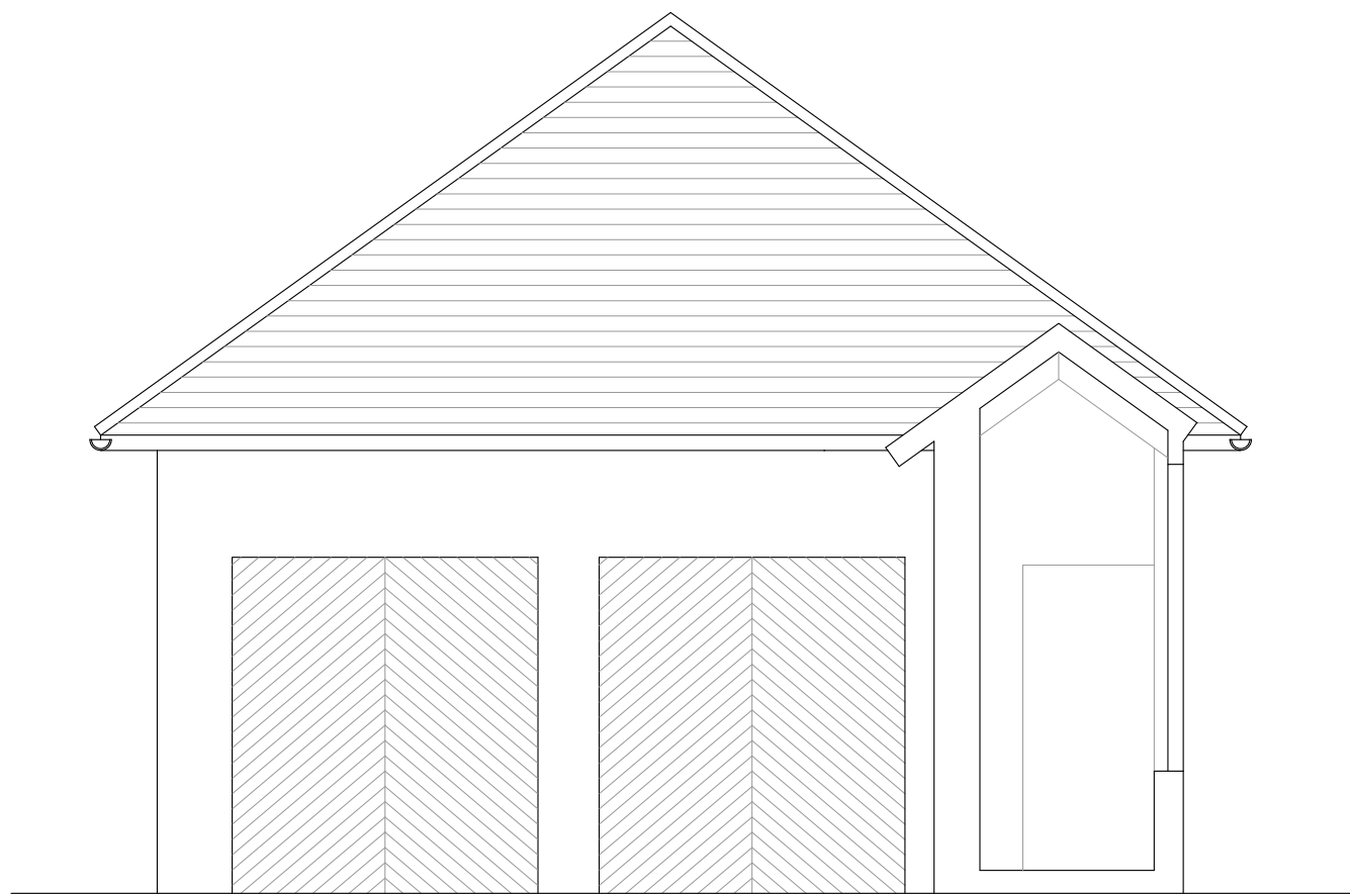
Side (West) Garage Elevation as Existing
