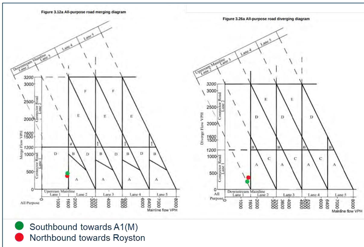
Figure 2-17: Merge/Diverge Comparison
