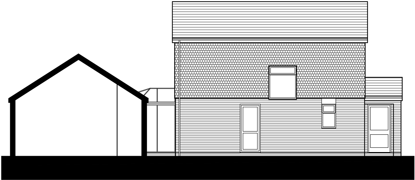
SIDE ELEVATION (B-B)
