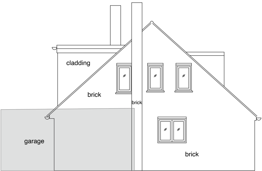
Elevation 2 (Side)
