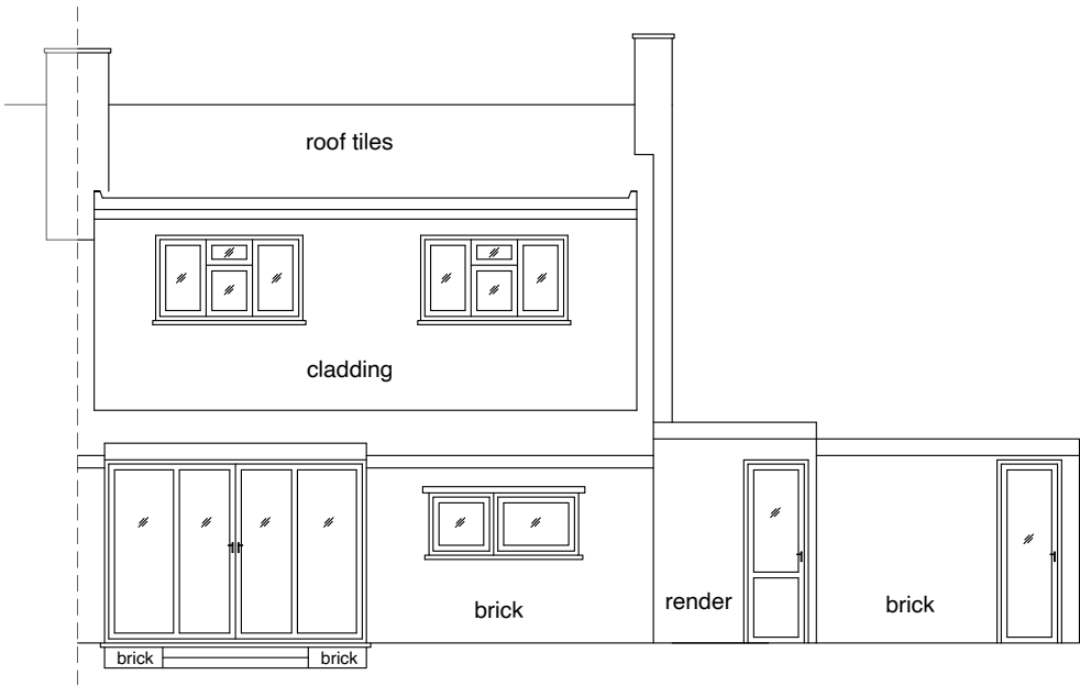
Elevation 3 (Rear)
