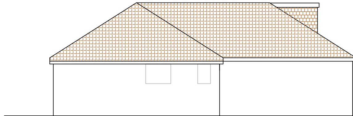
PROPOSED SIDE VIEW
