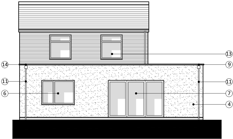
REAR ELEVATION (C-C)
